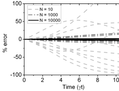
Figure 3.3.: The error in % is shown of the Monte Carlo simulation compared to the analytical decay curve. Shown are 10 realisations of ensembles consisting of N = 10 , 1000 and 10000 respectively for the light grey dashed, the grey dash-dotted and the black solid lines. The time axis is normalised to the decay rate in a homogeneous medium.
