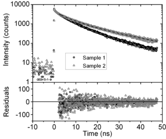
Figure 2.7.: Decay curves for quantum dots samples with different SiO 2 layer thicknesses, z = 73 nm and z = 166 nm respectively for sample 1 and 2, measured at an emission energy of 2.08 eV. The decay curves are fitted with a lognormal distribution of decay rates. Residuals are shown in the bottom panel.
