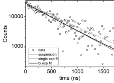
Figure 4.11.: The decay curve of quantum dots measured in a photonic crystal is shown. The lines are decay in suspension (light grey), a single exponential fit to the data (grey line) and a bi-exponential fit (black line). In this case a=1 , b=0.77 and I_0=16103 .
