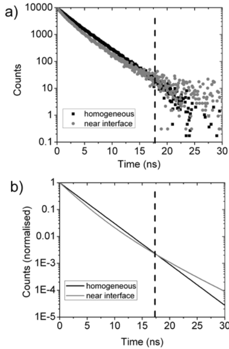
Figure 3.4.: a) The measured decay curves for R6G in a homogeneous medium and 10 nm from an n = 1.52/n = 1 interface (black and grey data respectively). b) The calculated decay curves for an ensemble of emitters in the experimental configuration. The vertical dashed lines indicate the intersection of the exponential and non-exponential curves.
