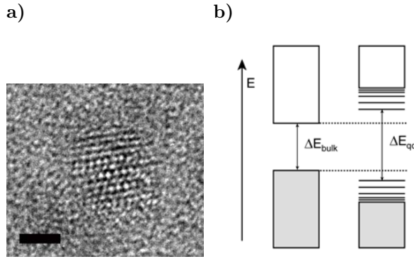
Figure 1.4.: a) A transmission electron microscope image of a CdSe quantum dot is shown. The scale bar is 2 nm. b) The band structure for bulk semiconductor and quantum dots is shown schematically.
